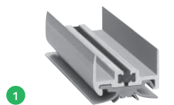
1 Bottom channel has thermal break and runs entire width of door.
