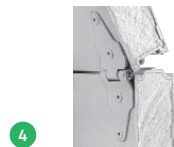
4 PVC thermal break connects front and back of door. No thru-metal areas to conduct heat or cold through the door.
